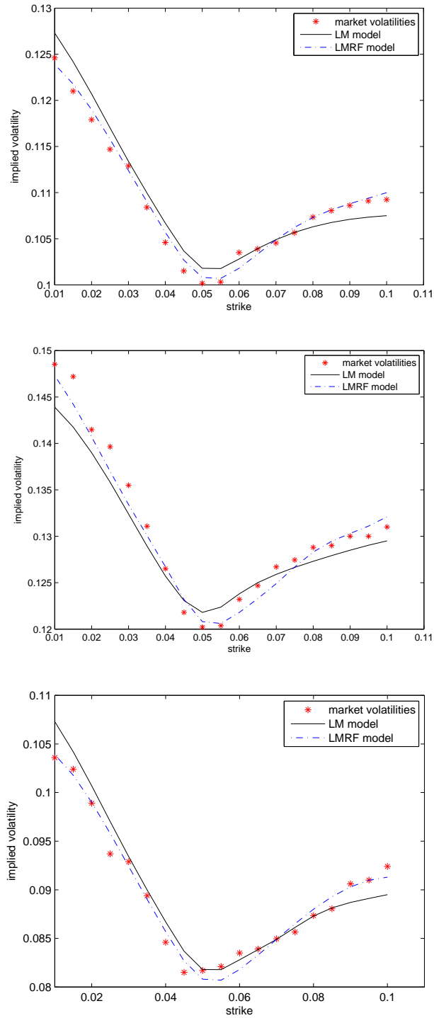
Figure 1: Examples of Caplet Volatility Smile Calibration for Maturity 1 year, 3 years, 15 years.
